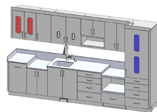
86" x 144" x 25 3/4" (HWD) 12' Sterilization Center Standard Configuration PN: 300-1012
