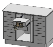
80" x 73 11/16" x 20" (HWD) Rear Delivery Extended workspace with 25" arm Putty tubing PN: 300-1321 Black tubing PN: 300-1321B
