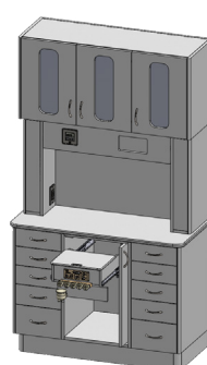
80" x 46 7/8" x 20" (HWD) Rear Delivery Upper cabinetry with 25" arm Putty tubing PN: 300-1320 Black tubing PN: 300-1320B
