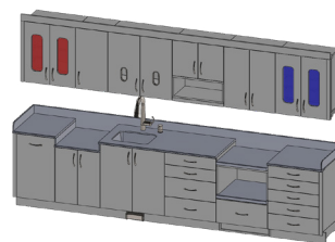
86" x 144" x 25 3/4" (HWD) 12' Sterilization Center Standard Configuration PN: 300-1112
