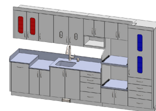
86" x 144" x 25 3/4" (HWD) 12' Sterilization Center Standard Configuration PN: 300-1312
